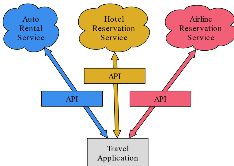
Service-oriented architecture
