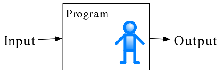
A Program
