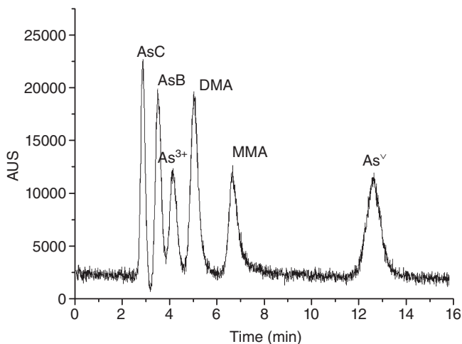
Fig. 12.5 HPLC-ICP/MS chromatogram of the six species of arsenic spiked in tissue sample (concentration: 40 \text{ ng} \cdot \text{g}^{-1} ).
