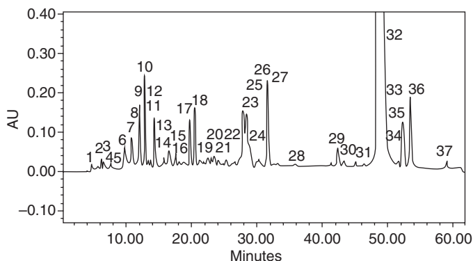
Fig. 10.8 HPLC-UV fingerprint of Qingkailing injection.
