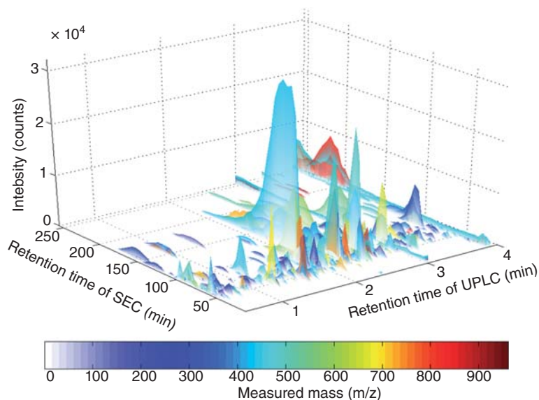
Fig. 3.7 Four-dimensional spectrum of HPLC \times UPLC-TOF/ MS system.
