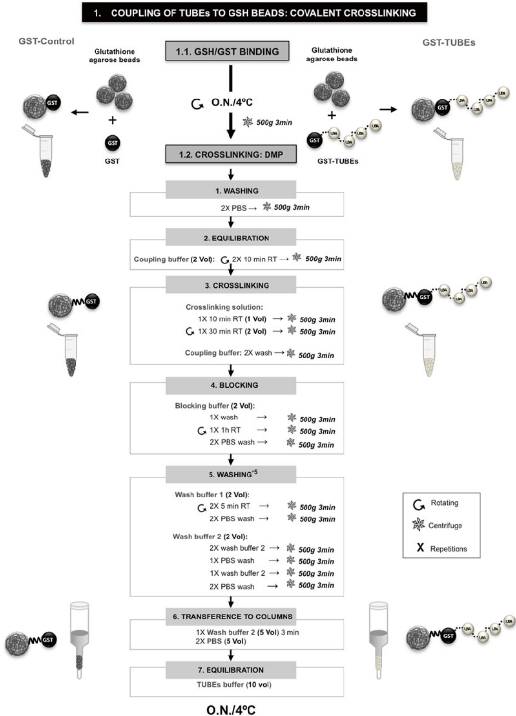
Fig. 1 Procedure to couple TUBEs/GST to GSH-agarose beads. Before covalent cross-linking using DMP, molecular traps were bound to agarose beads. After blocking active groups with ethanolamine, several washes are applied to eliminate unbound molecular traps and non-covalent interactions. Superscript numbers are associated to Subheading 4
