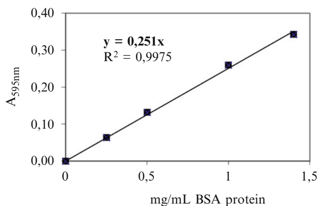
Fig. 2 Standard calibration curve for protein quantification from data obtained with the Bradford assay. The resulting linear regression equation is shown in bold. The y means the A_{595nm} while the x refers to the protein concentration
