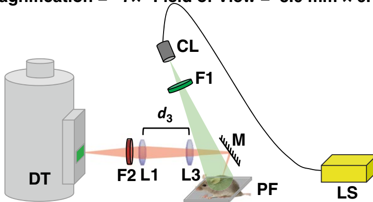
Fig. 2 Setups for in vivo NIR-II fluorescence imaging under different magnifications. (a) Optical diagram for in vivo NIR-II fluorescence imaging with a field of view of 60 × 48 mm that covers the entire mouse body, with d_1 = 0 mm. (b) Optical diagram for in vivo NIR-II fluorescence imaging with a field of view of 25 × 20 mm (~2.5× higher magnification than (a) ) that covers one of the mouse hind limbs or the entire mouse head, with d_2 = 200 mm. (c) Optical diagram for in vivo NIR-II fluorescence imaging with a field of view of 8 × 6.4 mm (~7× higher magnification than (a) ) that covers part of the mouse hind limb or part of the mouse brain, with d_3 = 150 mm. CL : collimator, DT : 2D InGaAs detector, F1 : excitation filter set, F2 : emission filter set, L1 : 200-mm lens, L2 : 75-mm lens, L3 : 150-mm lens, LS : 808-nm laser diode, M : mirror, PF : animal platform
