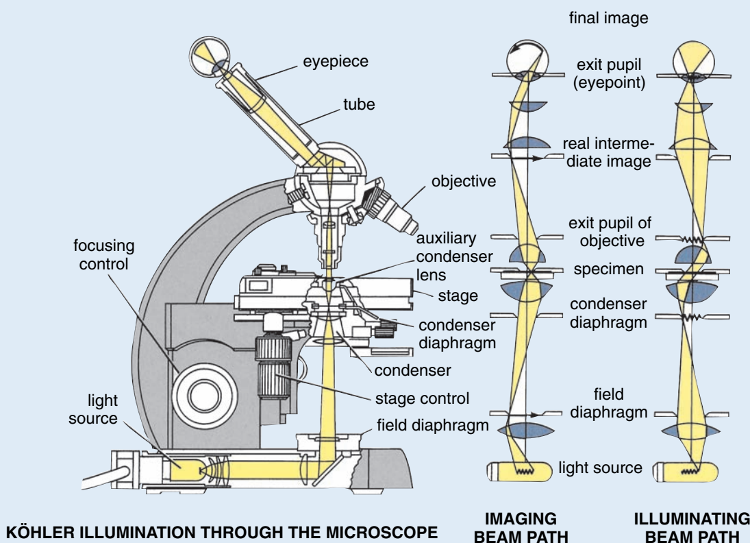
FIGURE F1.4.1 • Diagram of a typical light microscope. This drawing shows a cross-sectional view of the microscope, its operating components, and light path. (Courtesy of Carl Zeiss, Inc., Thornwood, NY.)
